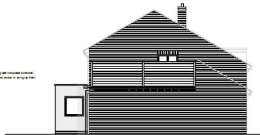
Proposed Side (West) Elevation
